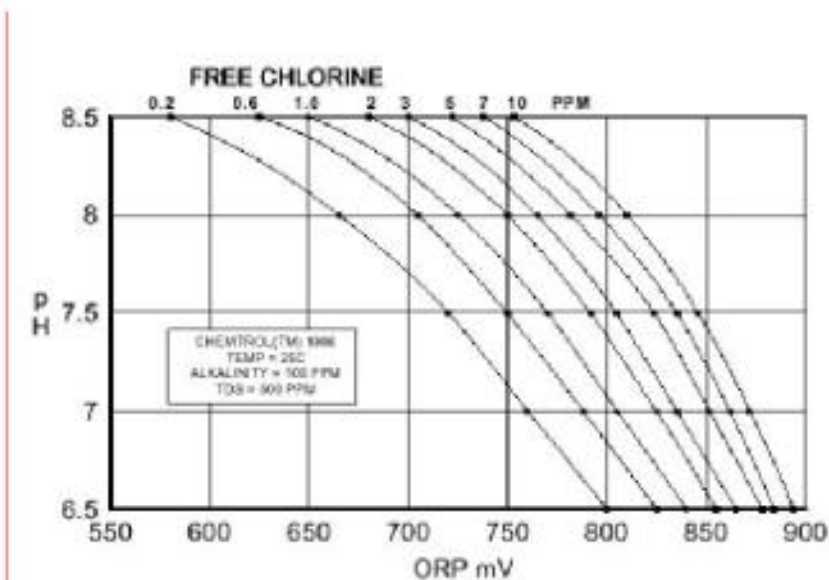
Figure 3 - PPM Readings vs. ORP and pH
